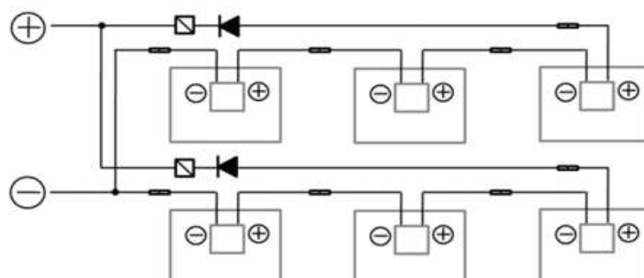
Fig.10-2 Parallel Connection
