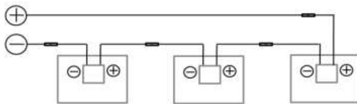
Fig. 10-1 Series Connection
