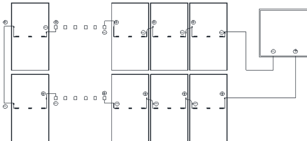
Fig. 9-2 Horizontal installation of short cable modules
